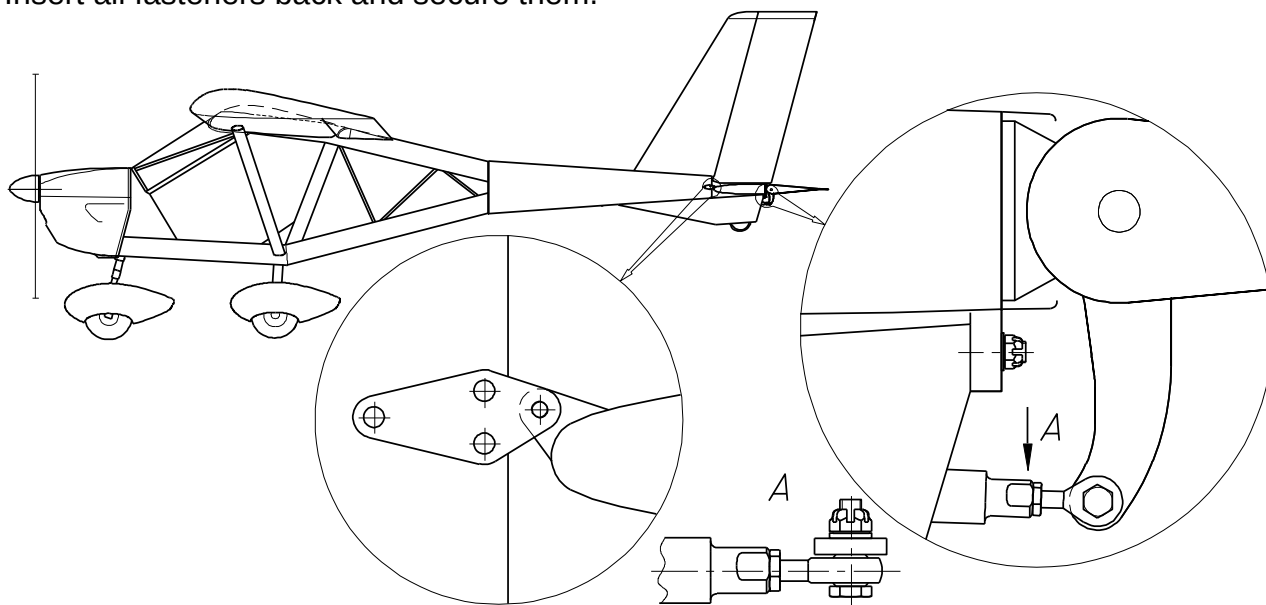
Fig. 22. Disconnection of the horizontal tail
