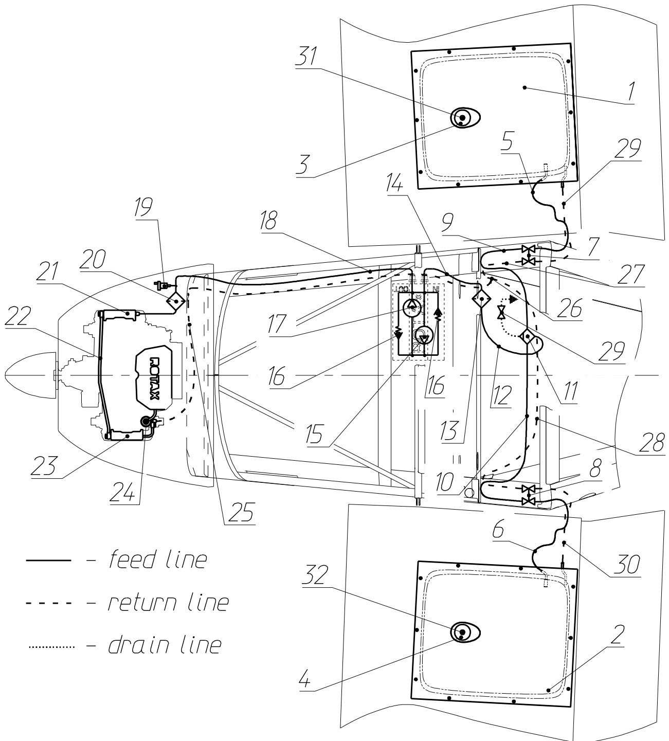
Fig. 3. Fuel system schematic
