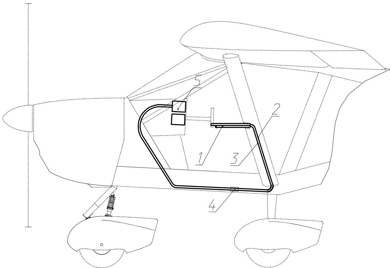
Fig. 12. Full and static pressure system
