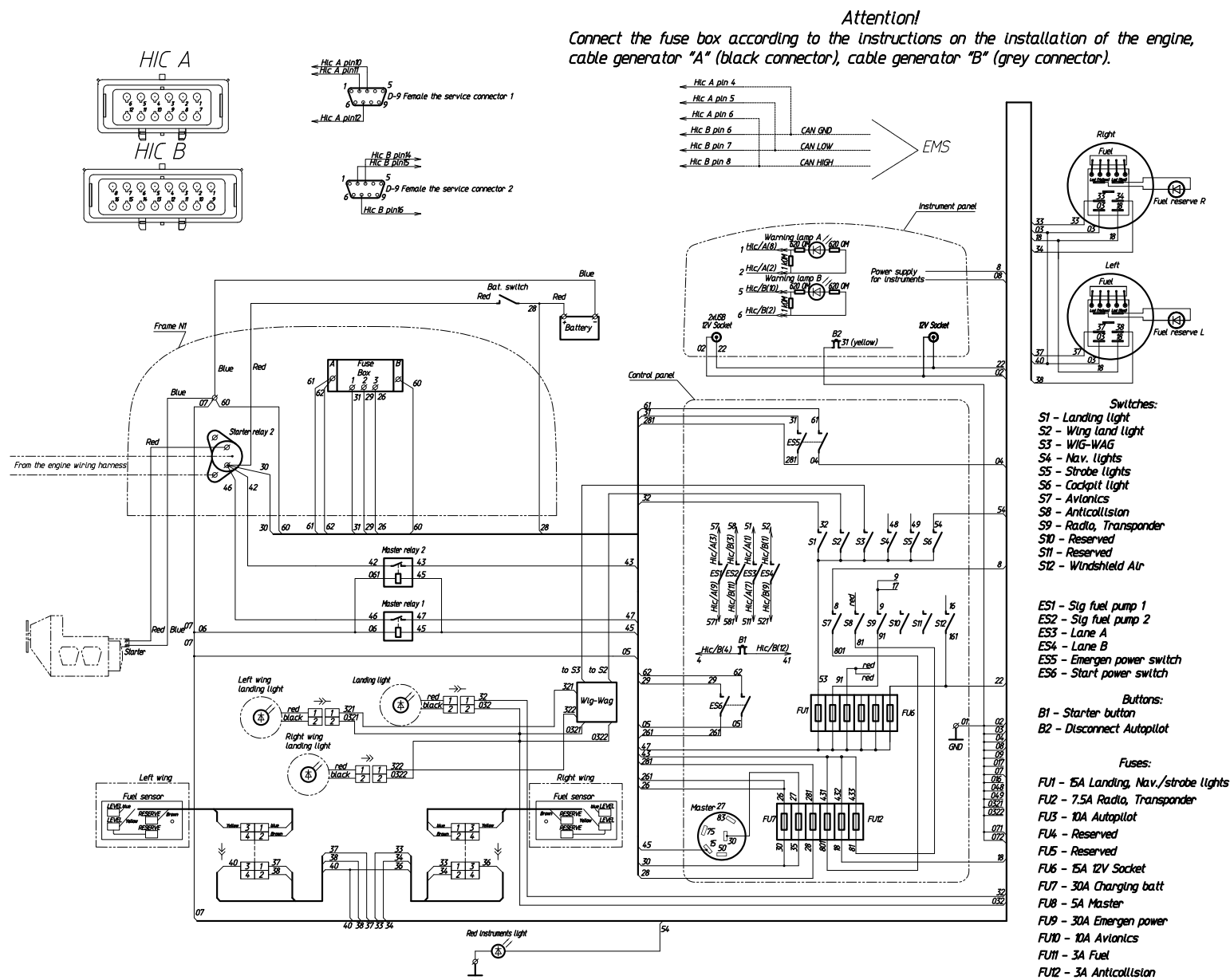
Fig. 13. Wiring diagram of A-22LS electrical system (main)
