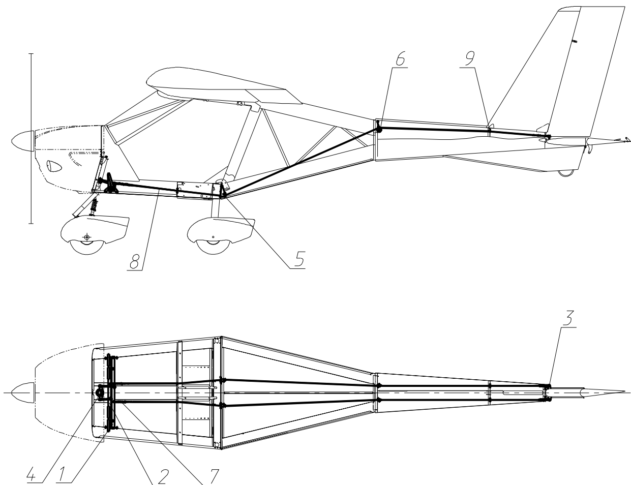
Fig. 6. Rudder and nose landing gear control system
