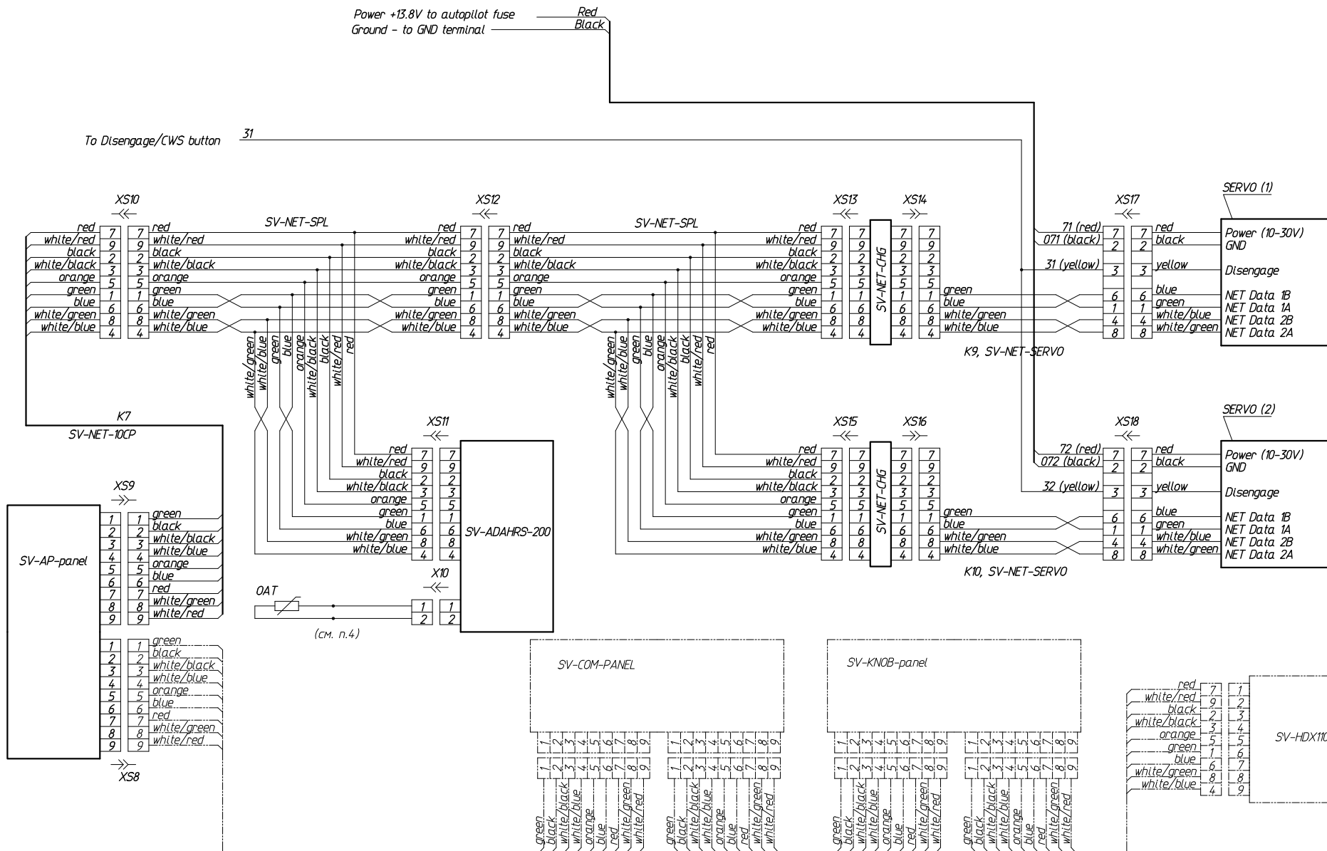
Fig. 16. Wiring diagram for installation of the Dynon Sky View system (sheet 3)
