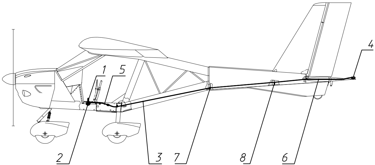
Fig. 5. Elevator trim tab control system
