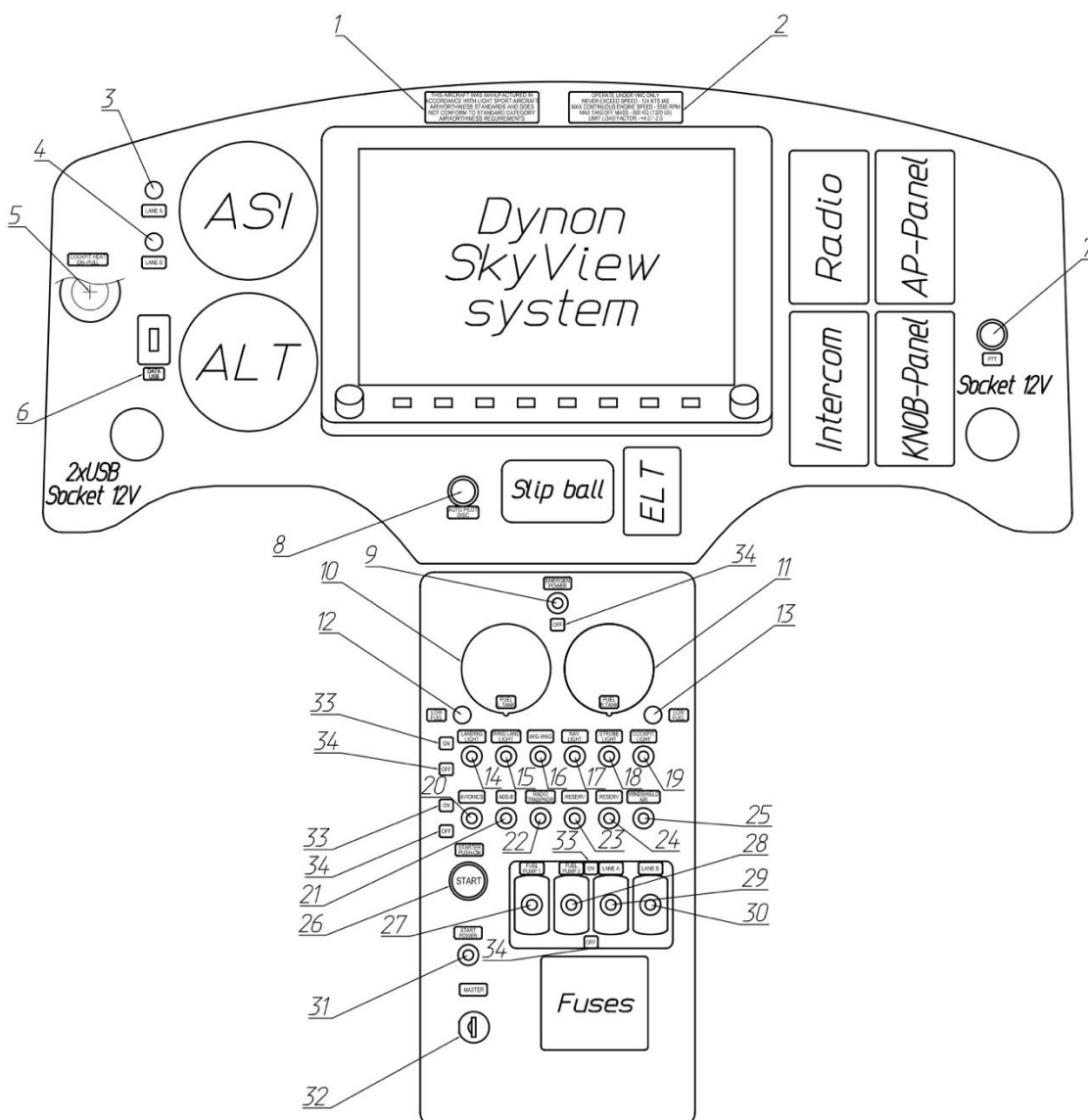
Fig. 11 Instrument panel
