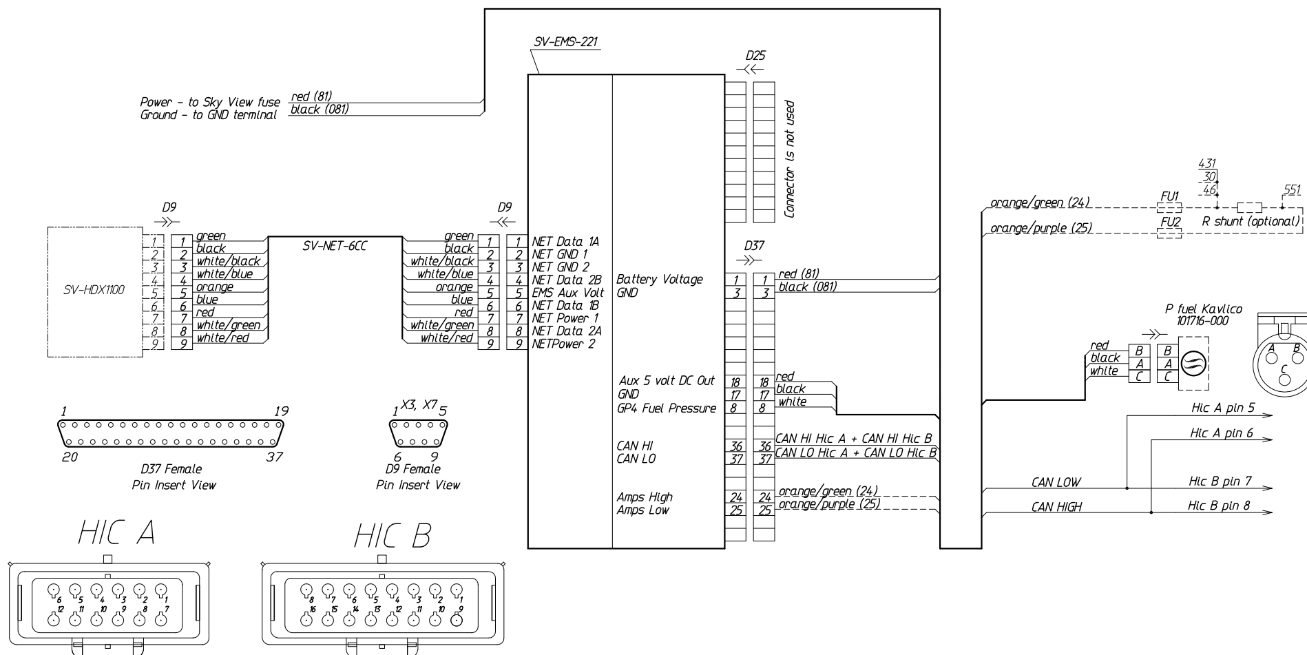
Fig. 14. Wiring diagram for installation of the Dynon Sky View system (sheet 1)
