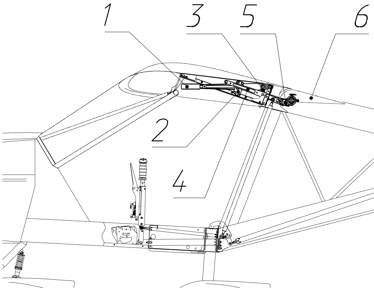
Fig. 8. Flap extension mechanism
