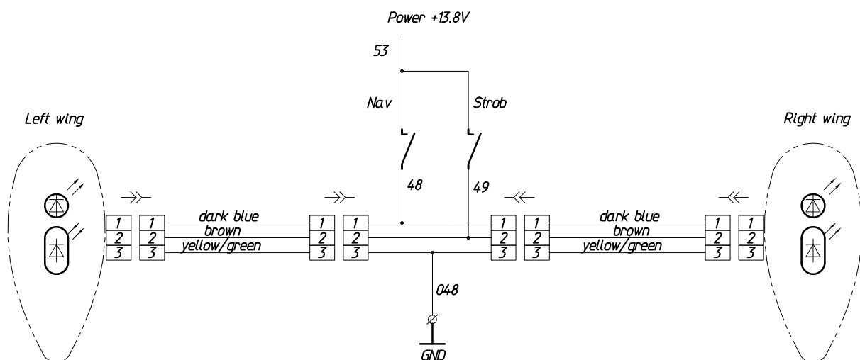
Fig. 20. Wiring diagram for installation of the navigation and strobe lights
